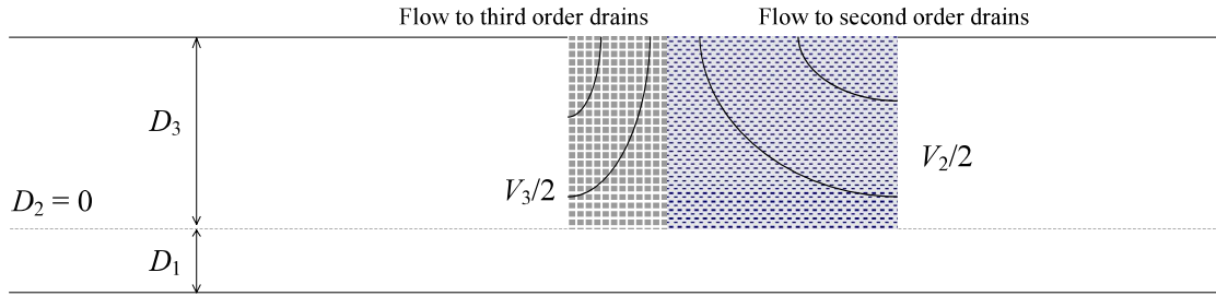
Figure B1.3 Schematization of regional groundwater flow to drains of three orders when either q_{\text{drain},1}L_{\text{drain},1} - q_{\text{drain},2}L_{\text{drain},2} < 0 or q_{\text{drain},2}L_{\text{drain},2} - q_{\text{drain},3}L_{\text{drain},3} < 0 .
