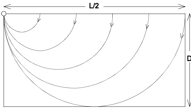
Figure B1.5 Flow field to a drain with half circular shaped stream lines.
